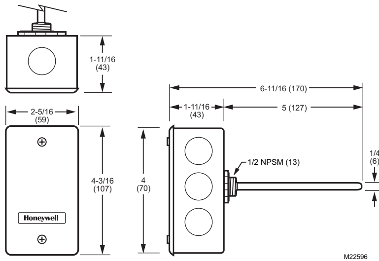
Fig. 5. C7021D, C7023D, C7031D, C7041D dimensions in in. (mm)
